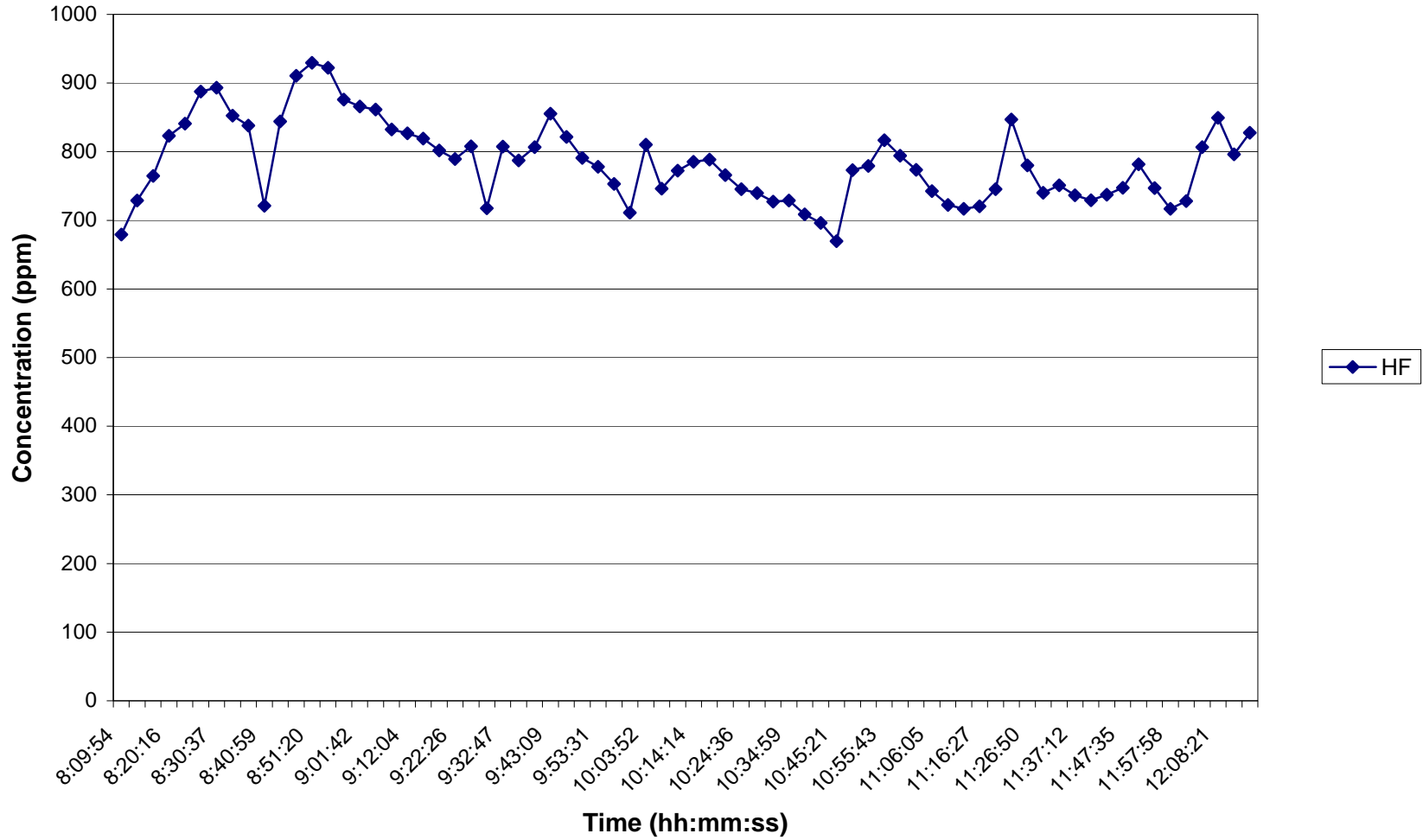
Time Series Plot for HF During HFC-134a Injection at 3600 ppm on 8/25/06
