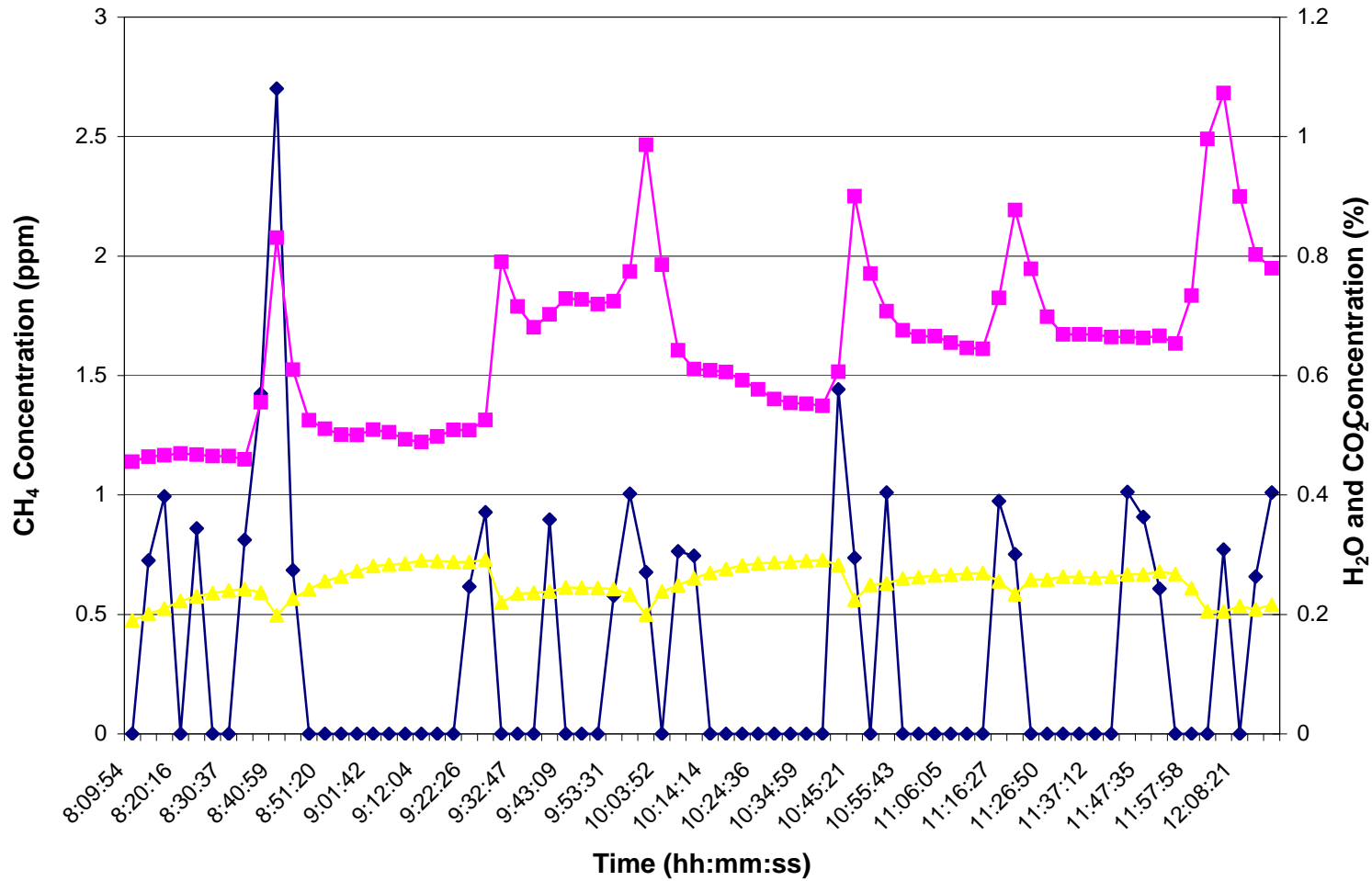
Time Series Plot for Ambient Air Compounds During HFC-134a Injection at 3600 ppm on 8/25/06
